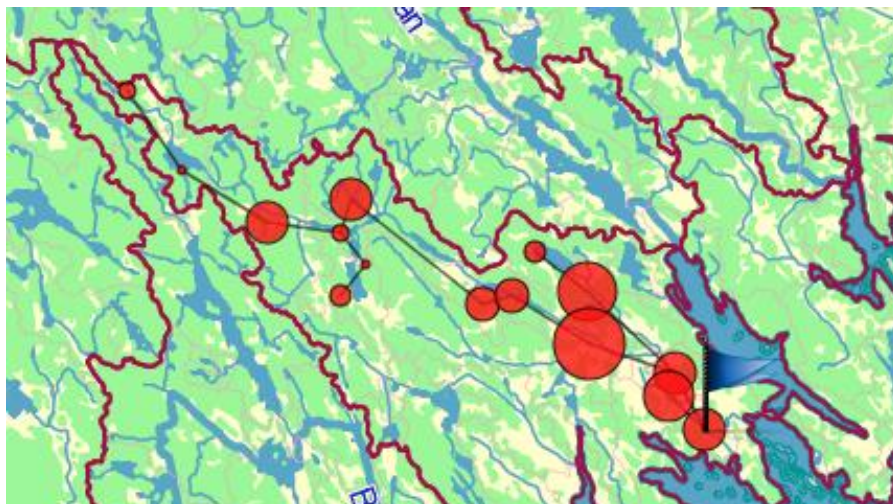
Nutrient load to Loftaån in different parts
